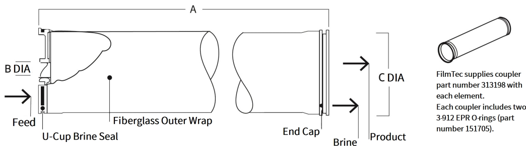
FilmTec™ Element BW30 PRO-400/34 Dimensions - inches (mm)
