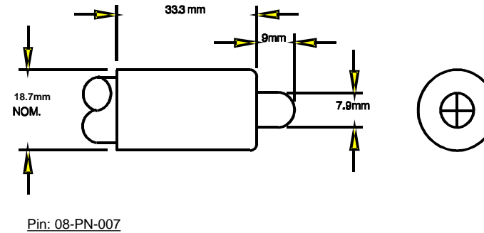
A08-60-CP0 HD Single Pin Base
