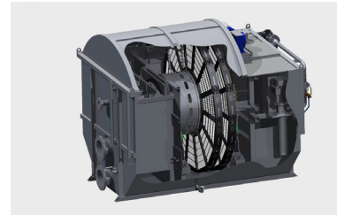
Forty-X™ Disc Filters
