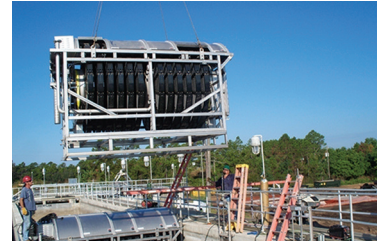
Upgrade or convert sand filtration to Forty-X™ Disc Filters
