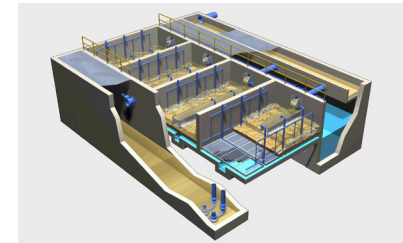
Hydro-Clear® Sand Filters
